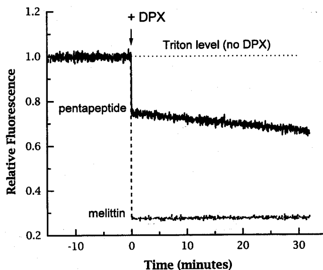
FIGURE 2 Reequenching kinetics of POPC vesicles originally loaded with ANTS and DPX and treated with the pentapeptide Ac-WLWLL or melittin. Vesicle suspensions containing 0.5 mM POPC were mixed with 0.14 mM pentapeptide (solid curve) or 0.4 \mu M melittin (dashed curve). After the fluorescence increase due to leakage had reached a plateau, additional DPX was added at the time designated t = 0 . Data are normalized to the fluorescence observed when the same amount of untreated vesicles were lysed with Triton X-100. Although in both cases DPX had apparently leaked completely as judged by fluorescence, the amount of released ANTS is clearly different, as indicated by the changes in the fluorescence levels for times greater than t = 0 . The smaller immediate drop in intensity observed after addition of DPX for the Ac-WLWLL sample suggests that less ANTS was released compared to the amount released by melittin. The slow decline of fluorescence for t > 0 seen in the Ac-WLWLL sample may be a result of quenching of internal ANTS due to the back-flow of the externally added DPX into the vesicles. These results demonstrate the existence of graded preferential release of DPX over ANTS.
