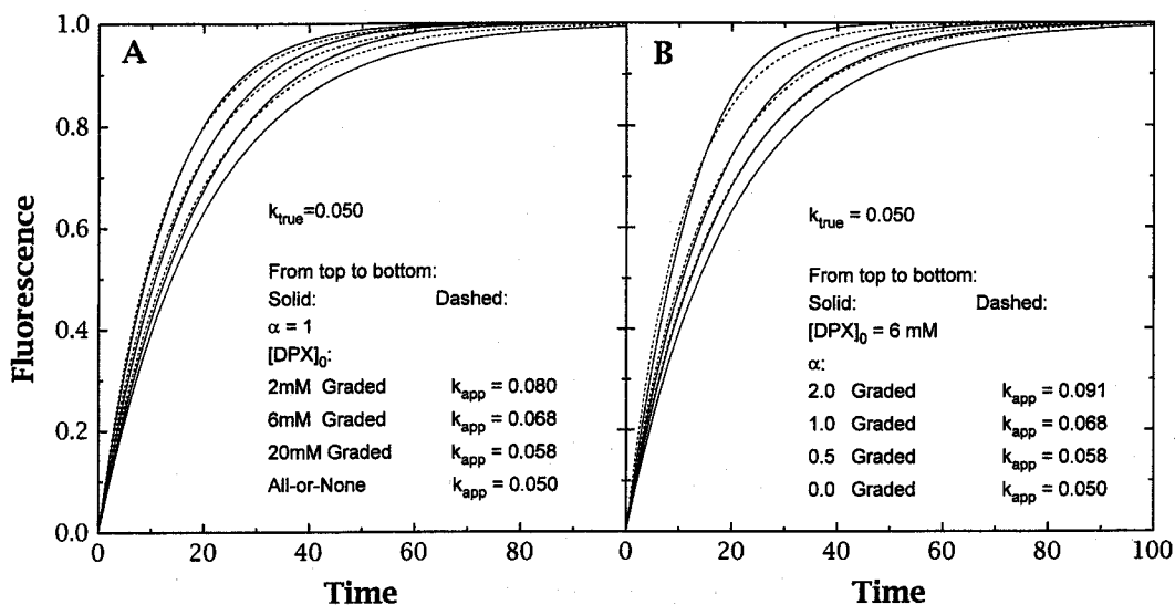
FIGURE 6 Fluorescence kinetics associated with the ANTS release with a rate k_{\text{true}} = 0.05 . (A) Nonpreferential leakage. (B) Preferential graded leakage. The solid curves show the fluorescence increases simulated using Eqs. 11 and 12 for the all-or-none and the nonpreferential ( \alpha = 1 ) graded leakage (A) and preferential graded leakage (B). The dashed lines correspond to the best fit of the exponential association model (Eq. 13), yielding an apparent rate k_{\text{app}} . In all cases of graded release, the kinetics of the fluorescence change became nonexponential. The apparent rate was always higher than the true rate of ANTS release, k_{\text{app}} > k_{\text{true}} . The fluorescence data follow the leakage exactly (lowest solid and dashed curves coincide) only when the release is all-or-none or when only ANTS is released in a graded fashion ( \alpha = 0 ). Note that for the case of nonpreferential graded release (A), which is realized for self-quenching dyes, the nonexponential behavior of fluorescence kinetics and its deviation from true leakage of material increase with the decrease of concentration of loaded marker.
