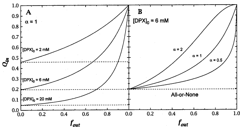
FIGURE 4 Simulations of internal quenching ( Q_{in} ) of ANTS inside vesicles as a function of the ANTS released ( f_{out} ). Dashed lines correspond to all-or-none release and solid lines to graded release simulated using Eq. 10. (A) The effect of initial DPX concentration for a nonpreferential release ( \alpha = 1 ). (B) The effect of preferential release. Because one is experimentally limited to f_{out} < 0.8 , both [\text{DPX}]_0 and \alpha affect one's ability to distinguish all-or-none from graded release in a reequenching experiment.
