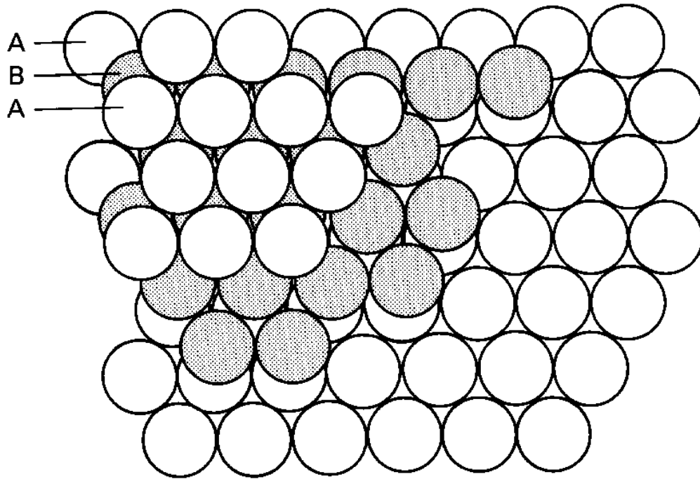
Hexagonal
