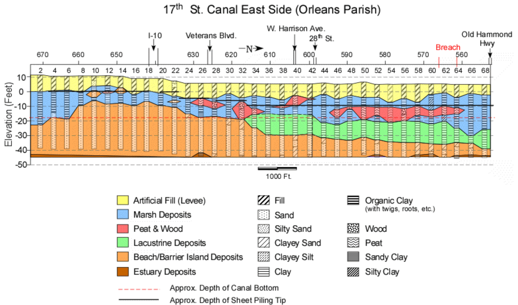
Figure 35. Geological cross-section along the eastern side of the 17 th St. Canal (based on data in the U.S. Army Corps of Engineers design documents (1990). Notable in the cross-section is the peat layer that occurs in the area of the breach.
