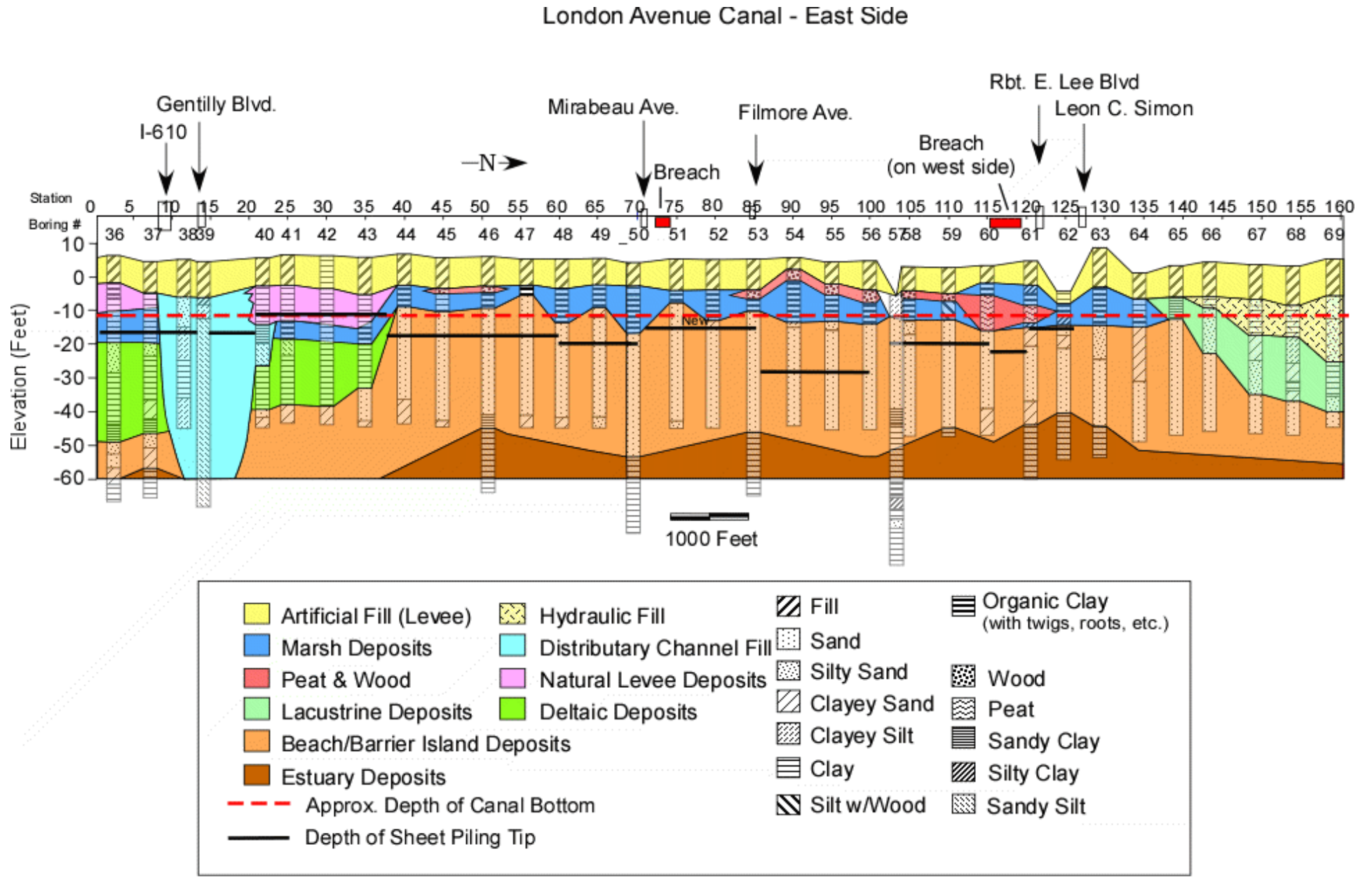
Figure 19. Geological cross-section along the east side of the London Avenue Canal constructed from data in U.S. Army Corps of Engineers (1989).
