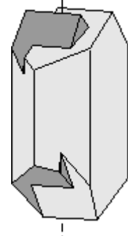
Twin Plane \{001\}
