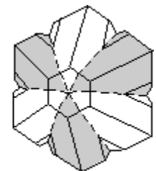
\{031\}
