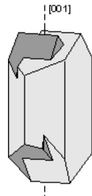
Twin Plane \{021\}
