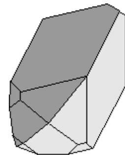
Twin Plane \{021\}
