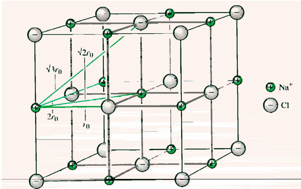
Figure 1.47 Sodium chloride structure showing internuclear distances.
