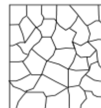
Phaneritic Texture
